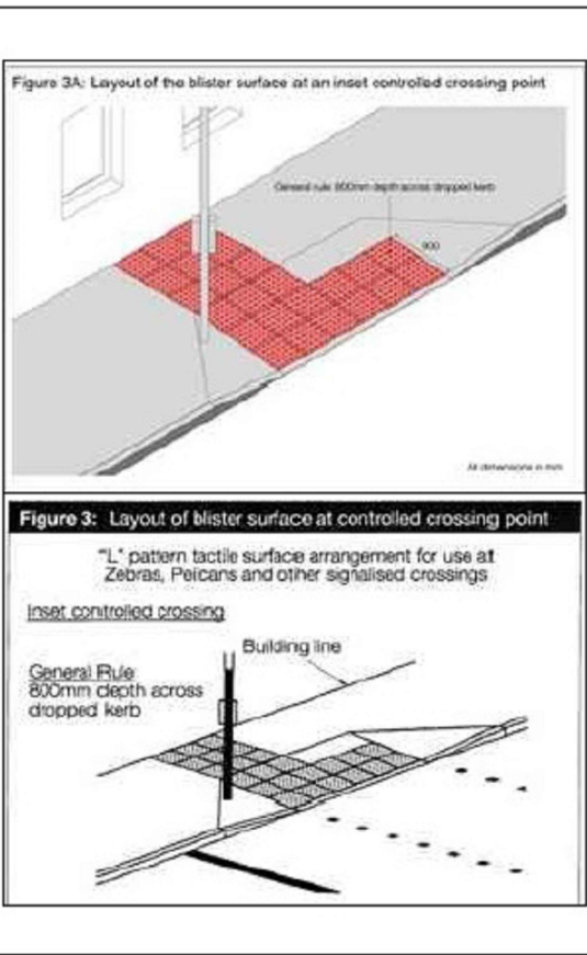
Standard detail for proposed road marking + tactile paving
